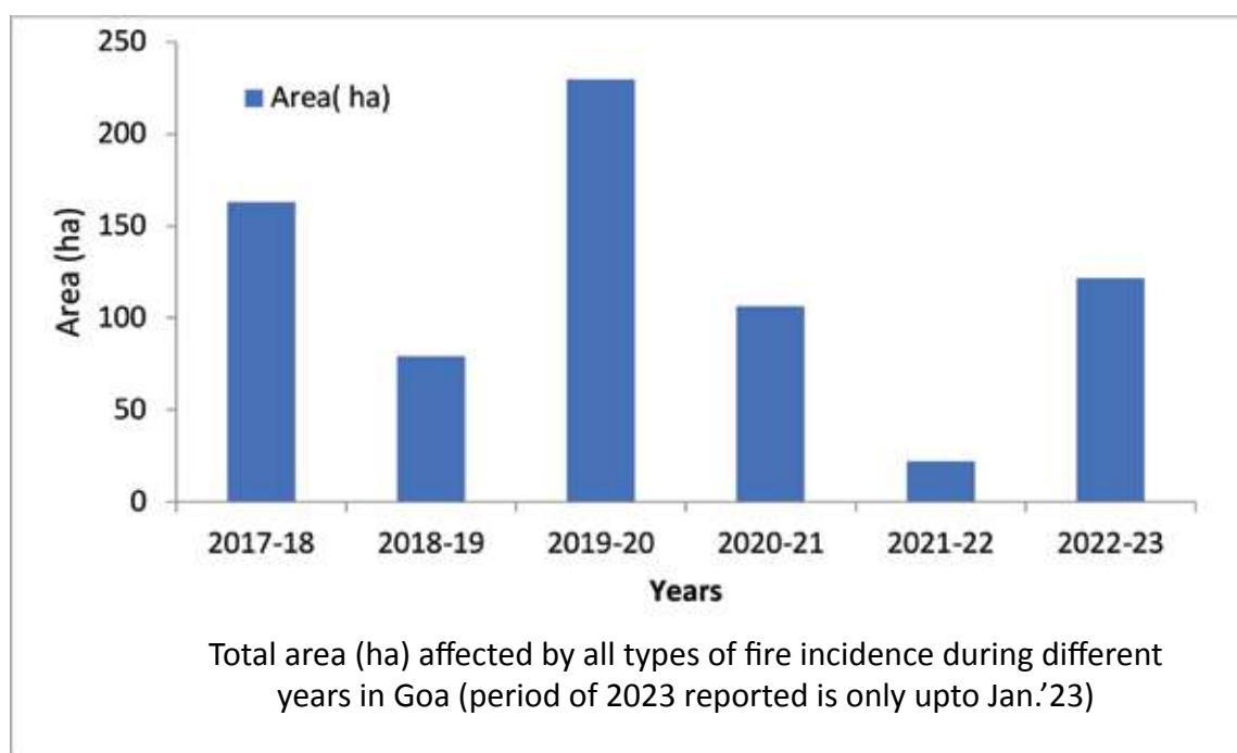
Fig. 6: Total area (ha) affected by forest fire in different years in Goa.
