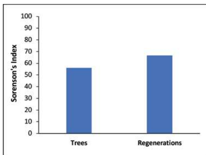
Fig. 7: Quotient of similarity of trees and regenerations in burnt and unburnt areas in different forest divisions of Goa
