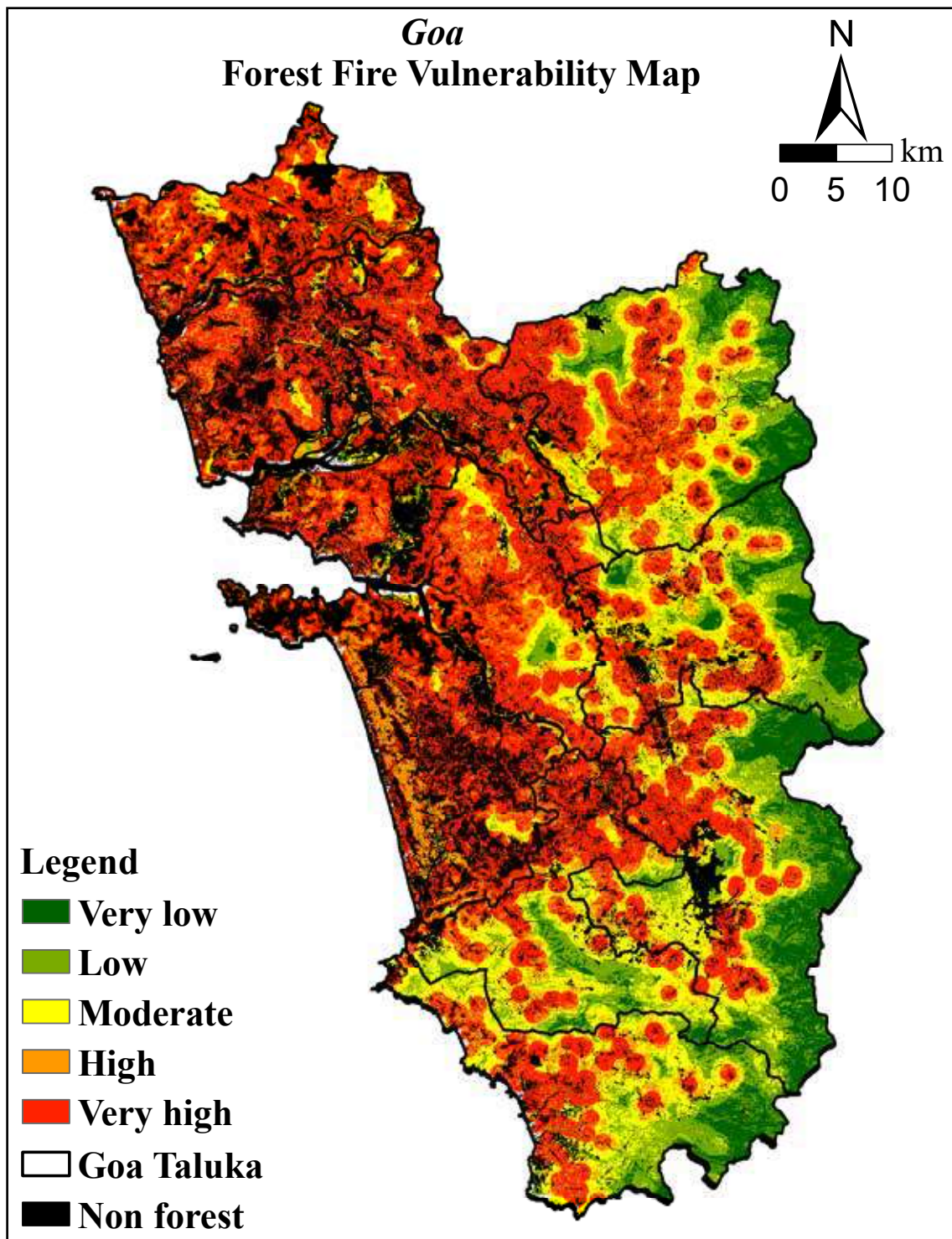
Fig. 15: Forest fire vulnerability map of Goa.
