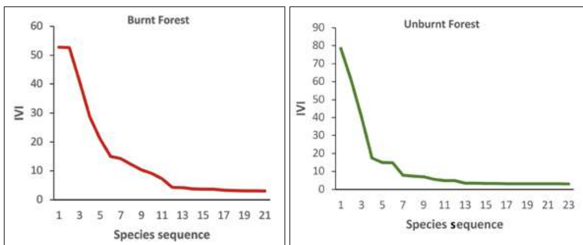
Fig. 11. Dominance diversity curve of tree species in burnt and unburnt areas in different forest divisions of Goa after the forest fire incidence of March-April, 2023
