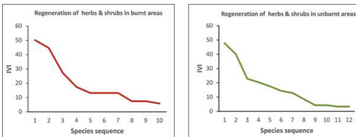
Fig. 10: Dominance diversity curve of regeneration of herbs and shrubs in burnt and unburnt areas in different forest divisions of Goa
