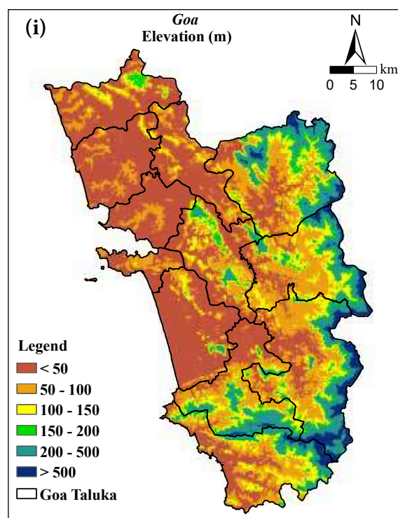
Fig. 14: The factors affecting forest fire vulnerability (a) distance from settlement, (b) distance from road, (c) forest types, (d) NDVI, (e) LST, (f) slope, (g) aspect, (h) TWI and (i) elevation.
