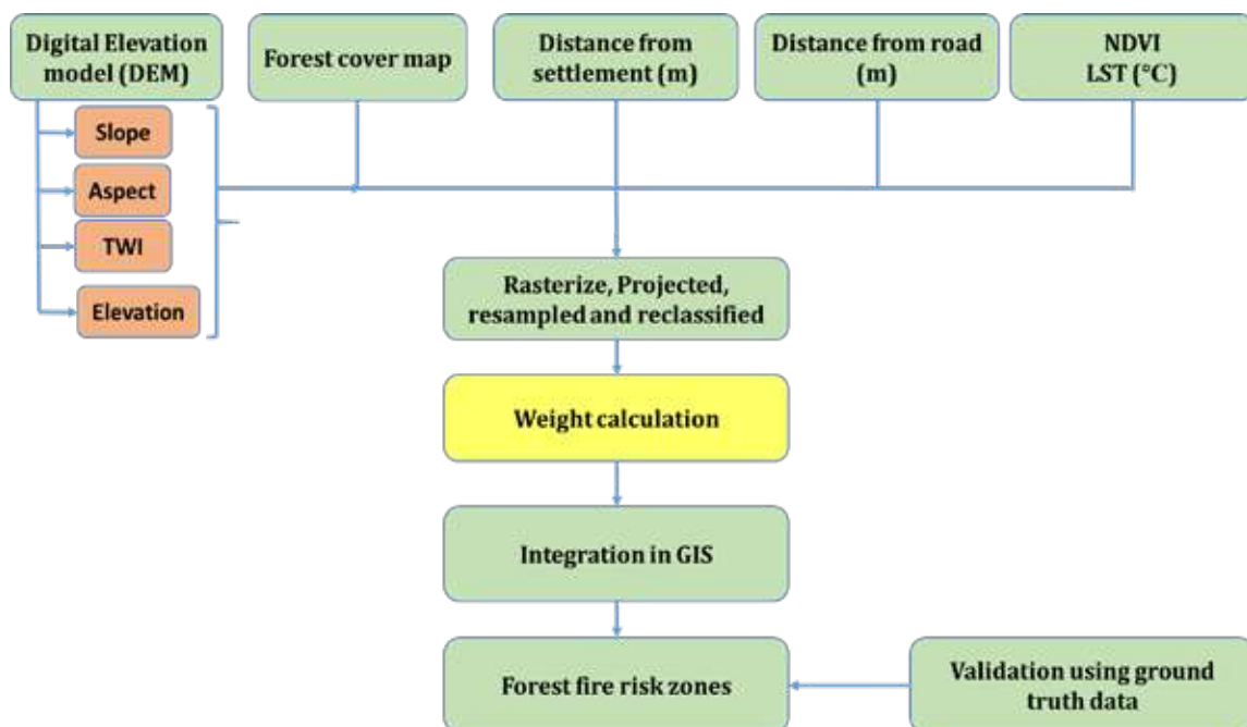
Fig. 5: Flow chart indicating procedure followed to prepare vulnerability maps.
