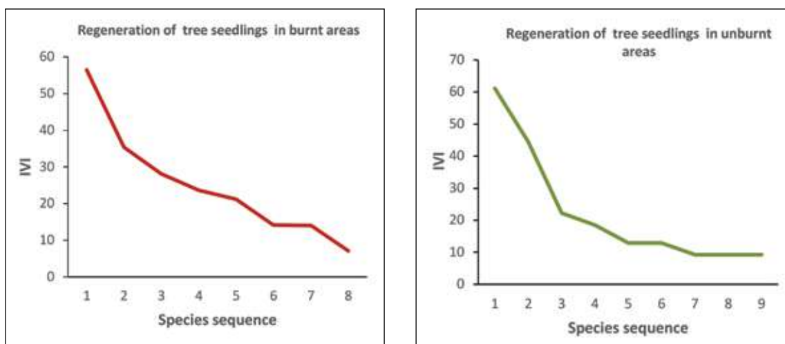
Fig. 9: Dominance diversity curve of regeneration of tree seedlings in burnt and unburnt areas in different forest divisions of Goa
