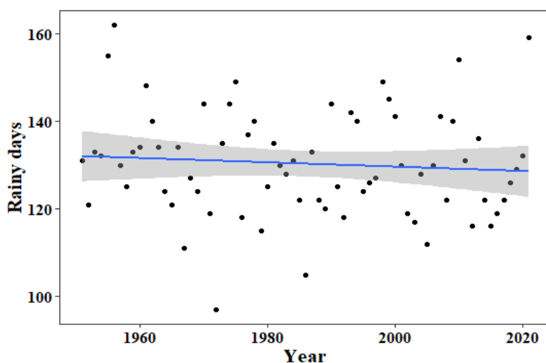
Fig. 4: Long term trends of number of rainy days in Goa.
