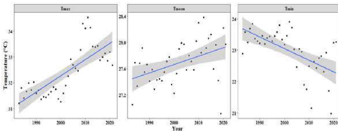
Fig. 2: Long term trends of max. and min temperature in Goa.
