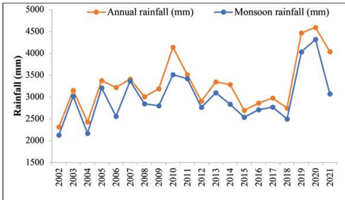
Fig. 1: Distribution of annual and monsoon rainfall in Goa over the last two decades.
