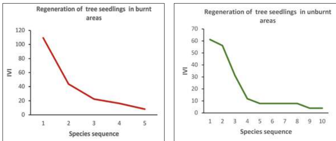
Fig. 12: Dominance diversity curve of regeneration of tree seedlings in burnt and unburnt areas in different forest divisions of Goa after the forest fire incidence of March-April, 2023
