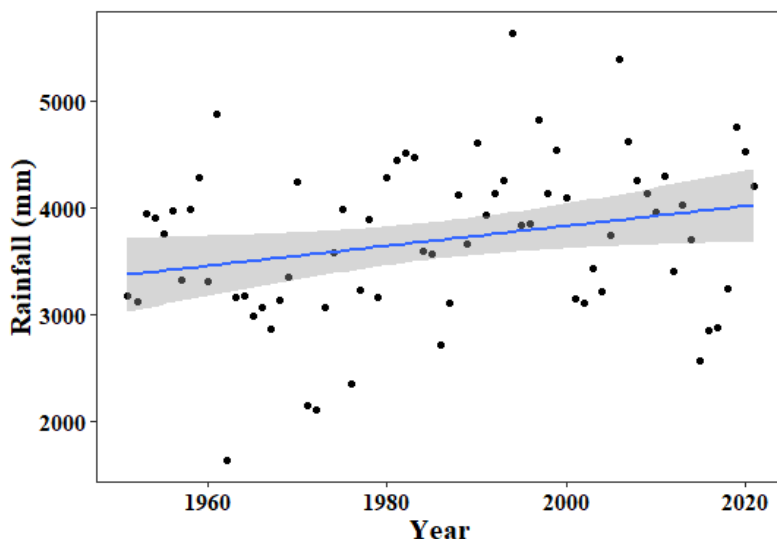
Fig. 3: Long term trends of annual precipitation in Goa.
