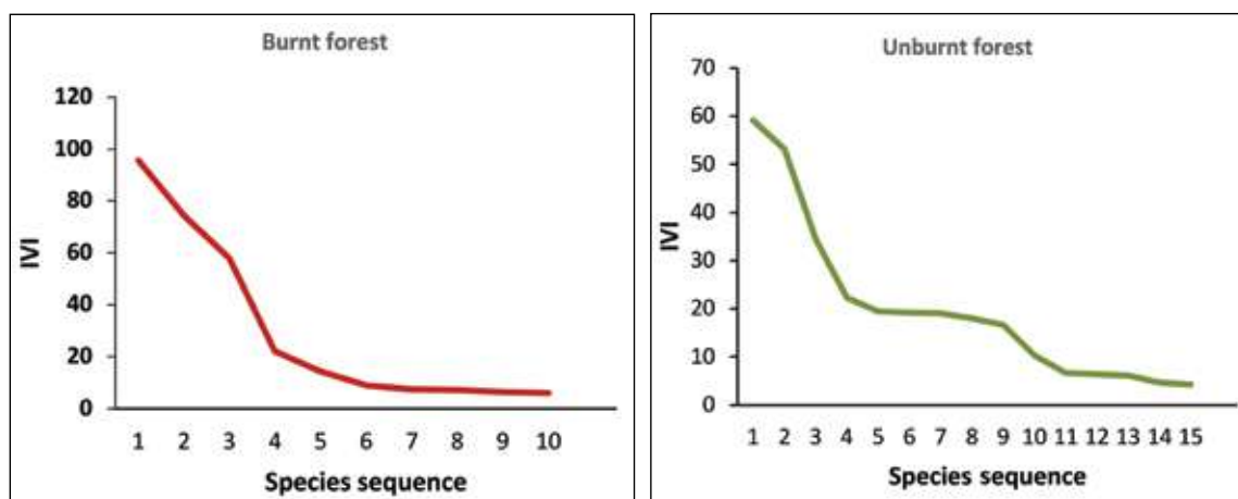
Fig. 8. Dominance diversity curve of tree species in burnt and unburnt areas in different forest divisions of Goa
