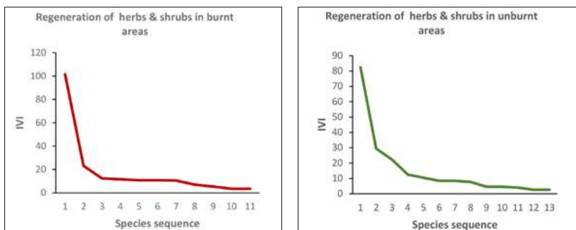
Fig. 13: Dominance diversity curve of regeneration of herbs and shrubs in burnt and unburnt areas in different forest divisions of Goa after the forest fire incidence of March-April, 2023
