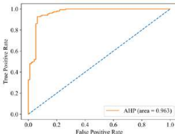
Fig. 16: ROC curve for the AHP-produced forest fire vulnerability map.
